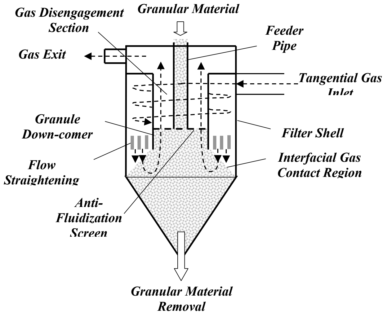
Figure 2. Operating principle of moving bed granular filter
