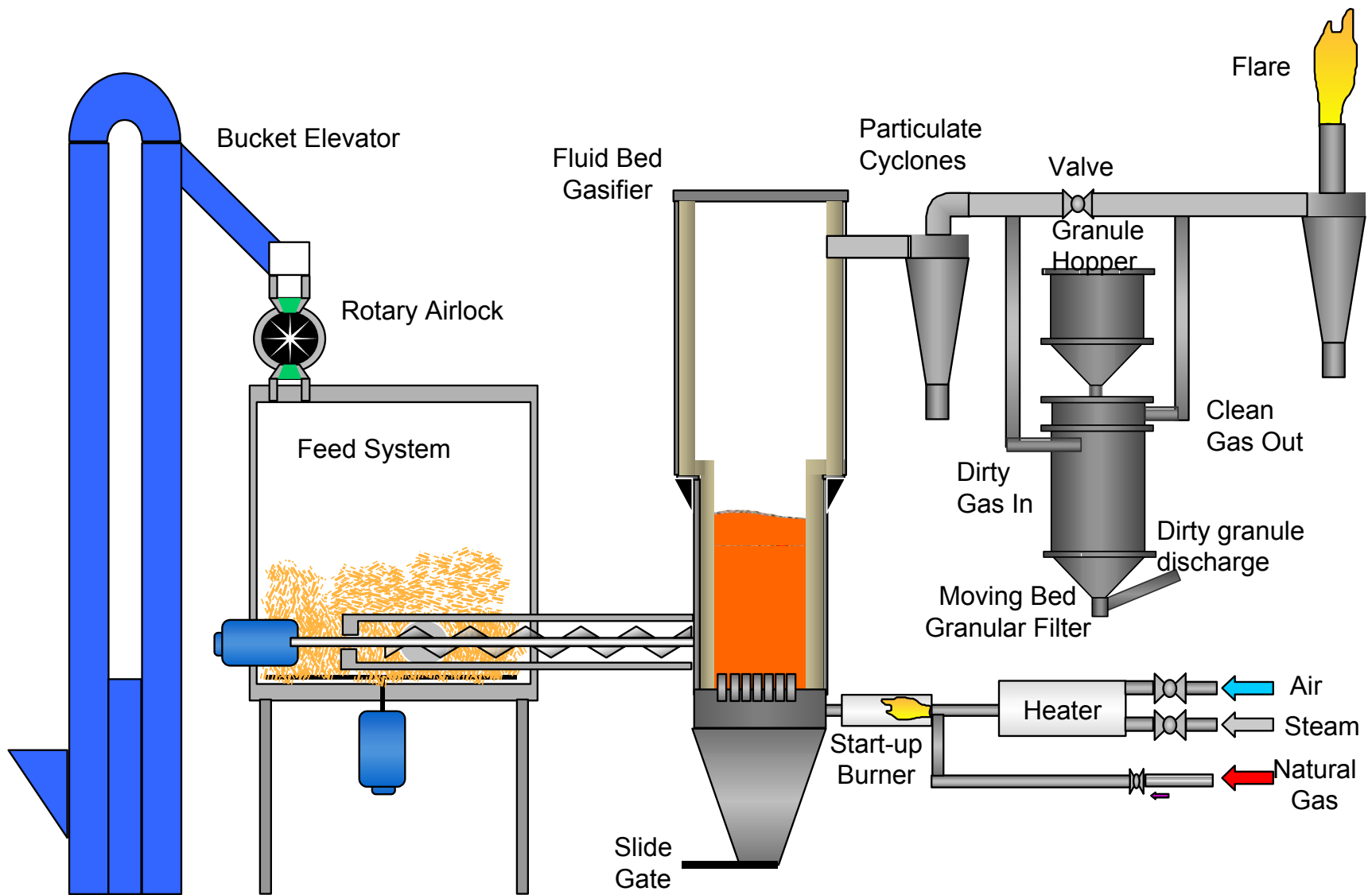
Figure 1. Schematic of fluid bed gasifier and moving bed granular filter.
